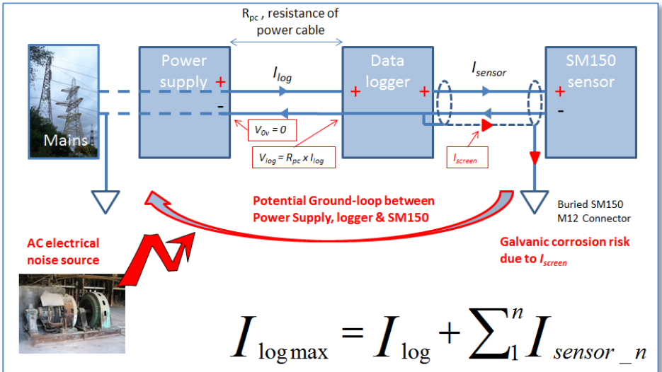
Figure 2 This diagrams shows that if the logger is are not well grounded then a potential ground loop can exist between the sensor and the power supply and/or mains power, and also the risk of galvanic corrosion to buried M12 connectors on the sensor and cable.
