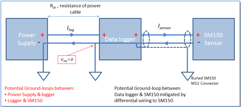
Figure 3 This diagram shows the logger, power supply and sensor all grounded. This minimises the possibility of galvanic corrosion of the SM150 connector. It also minimises the possibility of nearby AC-powered machinery injecting noise into the readings. The potential ground loop between logger and sensor is mitigated by the differential wiring of the SM150
